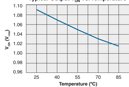
Typical Output V_{ON} vs. Temperature
